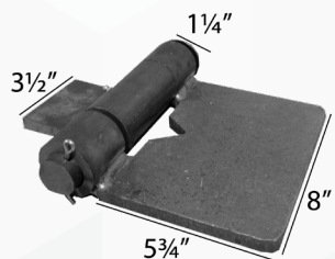
STANDARD TAILGATE HINGE 4040102
