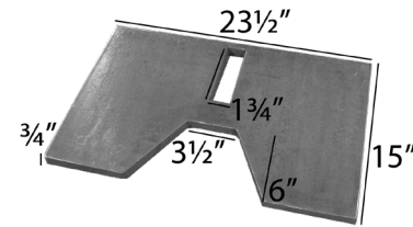
STANDARD ¾" HOOK PLATE 3120125
