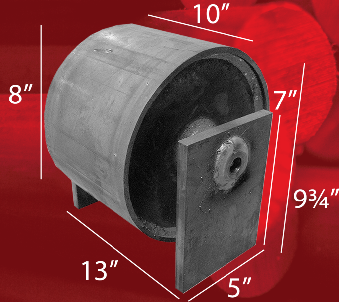
8" X 10" WHEEL WITH 5" X 7" BRACKET 4070120
