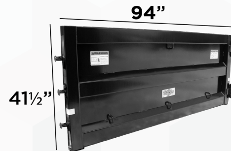
42"X94" 20YD TAILGATE 4050105
