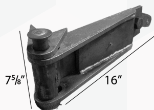
SEALED TAILGATE HINGE 4040104
