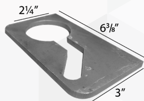
KEYHOLE BRACKET 3260104
