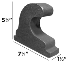
CABLE-STYLE HOOK 3120124
