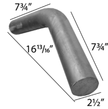
2½" HOOKLIFT PIN 3080128
