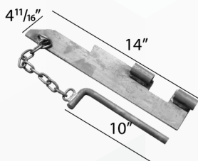
STANDARD LATCH BRACKET WITH PIN & CHAIN 4080106
